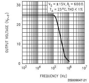
Power Bandwidth
