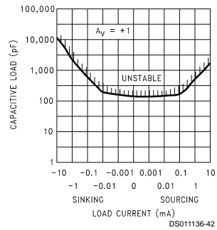
Stability vs Capacitive Load ( A_V = +1 )
