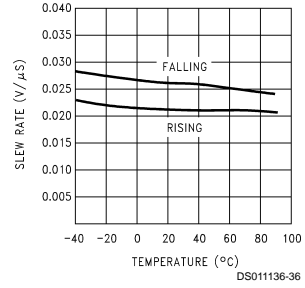
Non-Inverting Slew Rate vs Temperature
