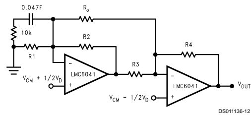
FIGURE 7. Two Op-Amp Instrumentation Amplifier
