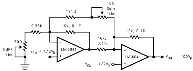
FIGURE 8. Low-Power Two-Op-Amp Instrumentation Amplifier
