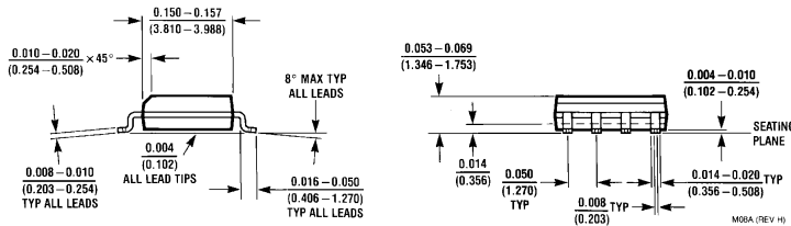
8-Pin Small Outline Order Number LMC6041AIM or LMC6041IM NS Package Number M08A
