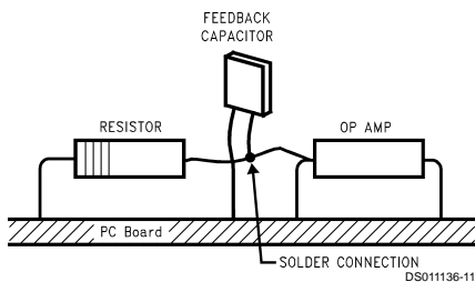
FIGURE 6. Air Wiring
