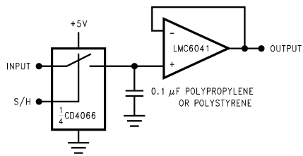
FIGURE 9. Low-Leakage Sample and Hold
